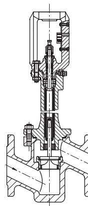
Fig. 6: Type 3241 Valve, forged steel version, DN 15 to 80, with bellows seal
