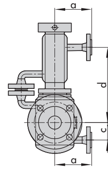
Bellows seal version with heating jacket
